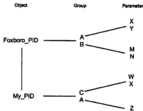
Figure 8 - Parameter Group Inheritance
